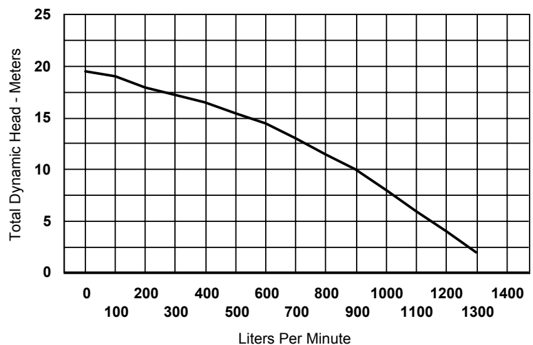
Piranha pump model P300-50 2.2 kw, 50 hz
