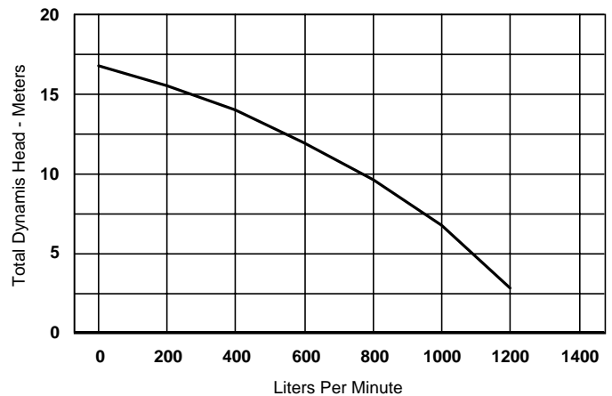
Piranha pump model PS1000A 7.5 kw 50 hz
