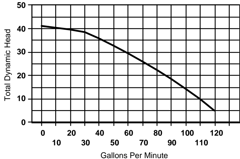
Piranha Pump Model PP-100 1 HP - 115 Volt 1 Phase
