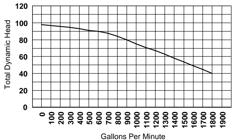
Piranha Agitator Pump Severe Duty Model P-50-A
