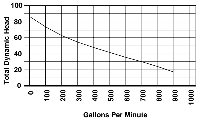
Piranha Solids Handling Pump Model PLS 1000
