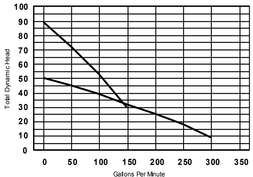
Piranha Model PP-250 HV & HH 2.5 HP -230/460 Vdt
