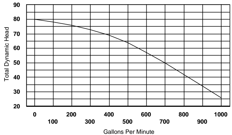
Piranha Agitator/Slurry Pump Model PS-2000-A
